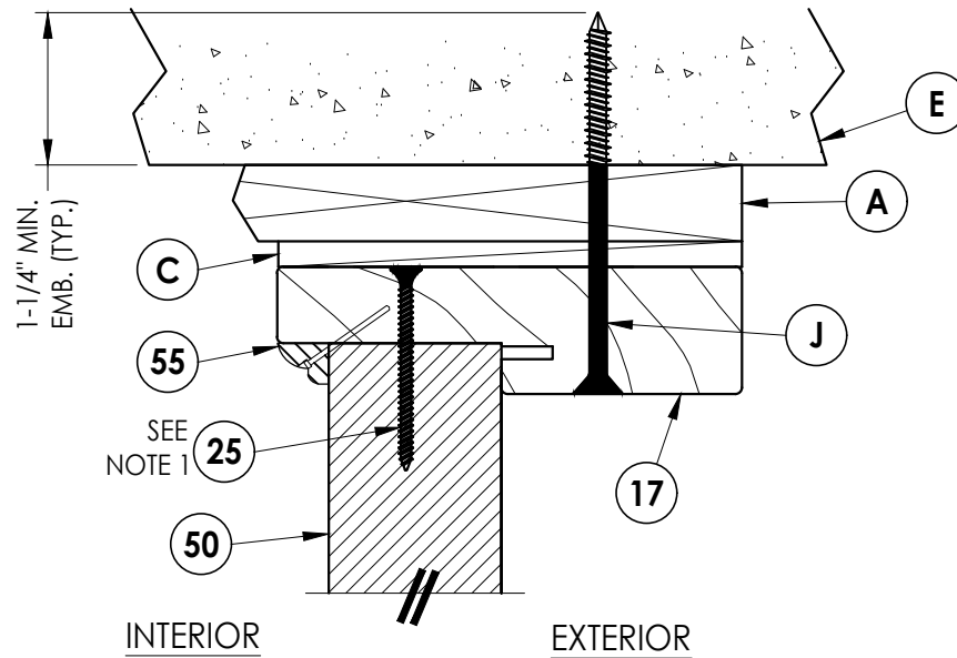
2 7 VERTICAL CROSS SECTION Shown w/1X sub-buck
